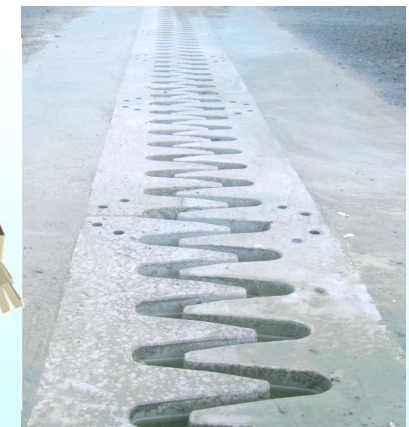
Expansion Joint & Other Utilities
